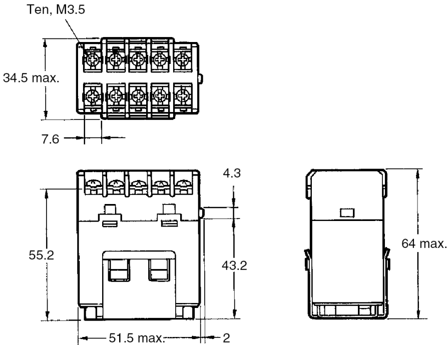
Outline drawing
